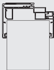
Telaio muro da 100/150 mm Wall frame from 100/150 mm
